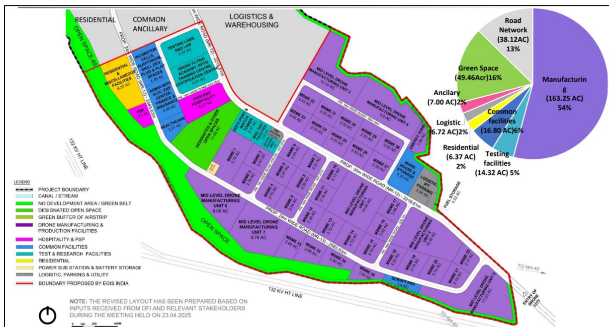
Figure No.2 – Drone City masterplan
